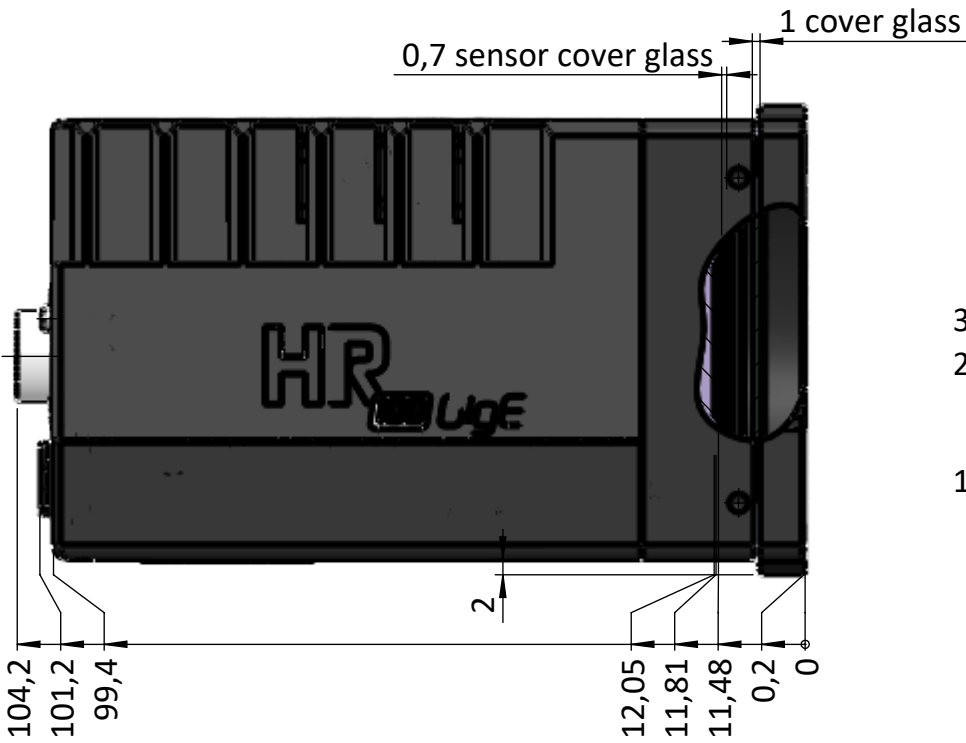
left view
